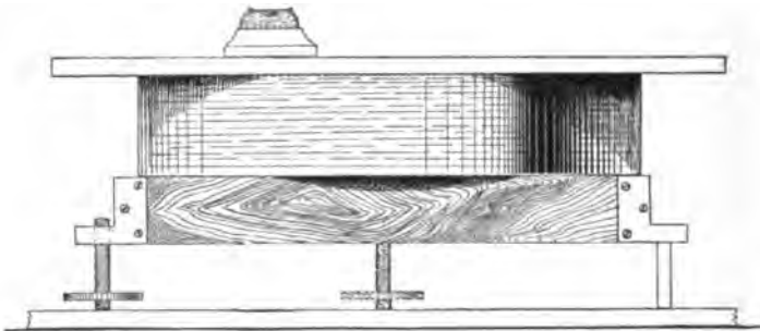
FIG. 123.—Plate-levelling stand, side view.
